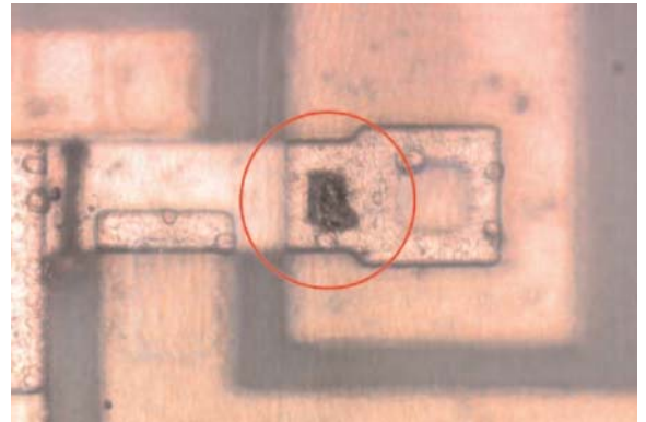
The MicroPoint laser provides deprocessing/removal of passivation and other materials for probing at the smallest sites.
