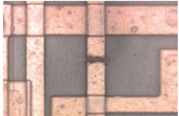
Circuit isolation can be achieved on diffraction limited structures and at specific levels of integration without any collateral damage
