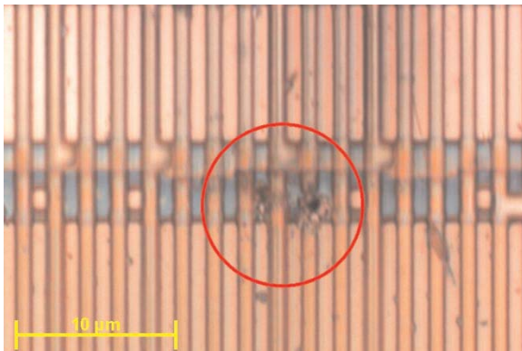
Circuit isolation can be achieved on diffraction limited structures and at specific levels of integration without any collateral damage
